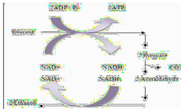
Figure 4: Conversion of a glucose molecule into two molecules of pyruvates and then pyruvate into ethanol with the circulation of energy in the form of ATP and NADH.
