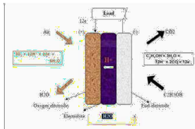
Figure 5: Direct ethanol fuel cell (DEFC) for the production of electricity from chemical energy.
